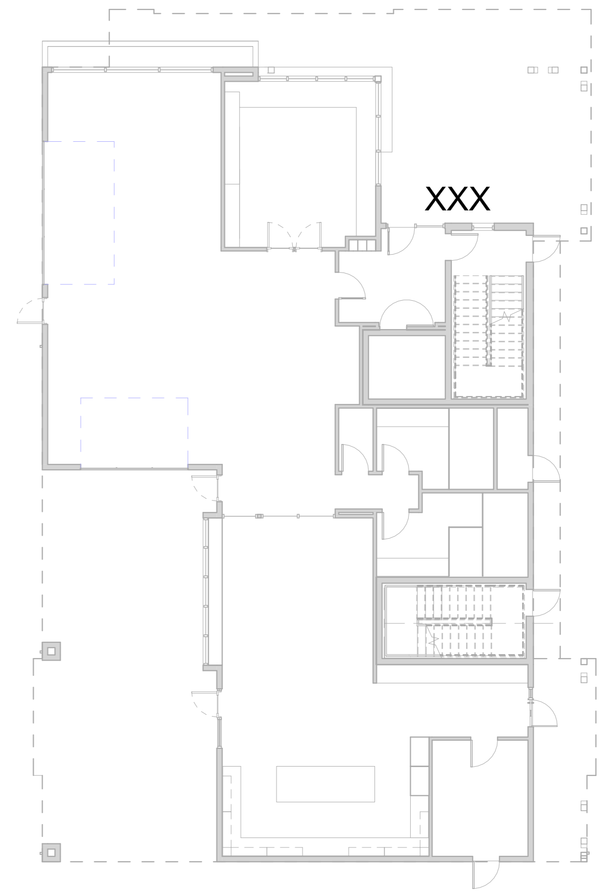
1 ADDRESS PLAN - LEVEL 1 3/32" = 1'-0"
