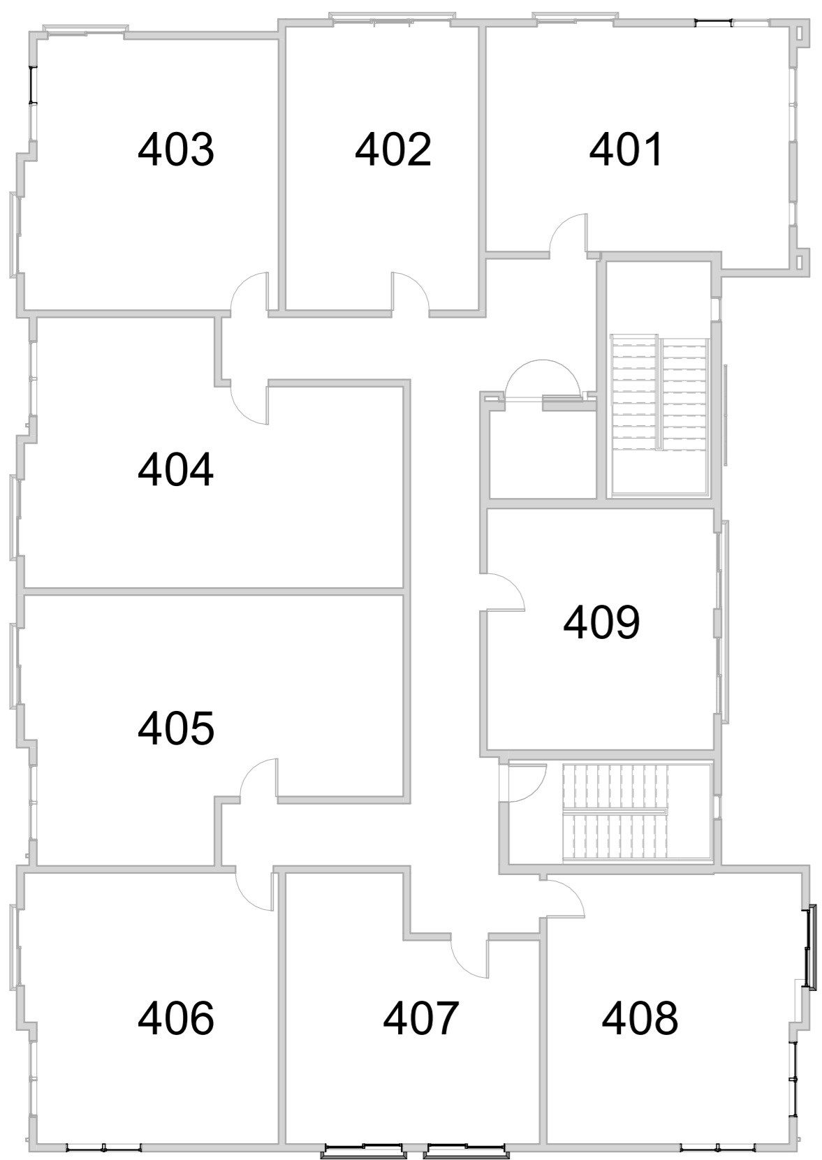
4 ADDRESS PLAN - LEVEL 4 3/32" = 1'-0"
